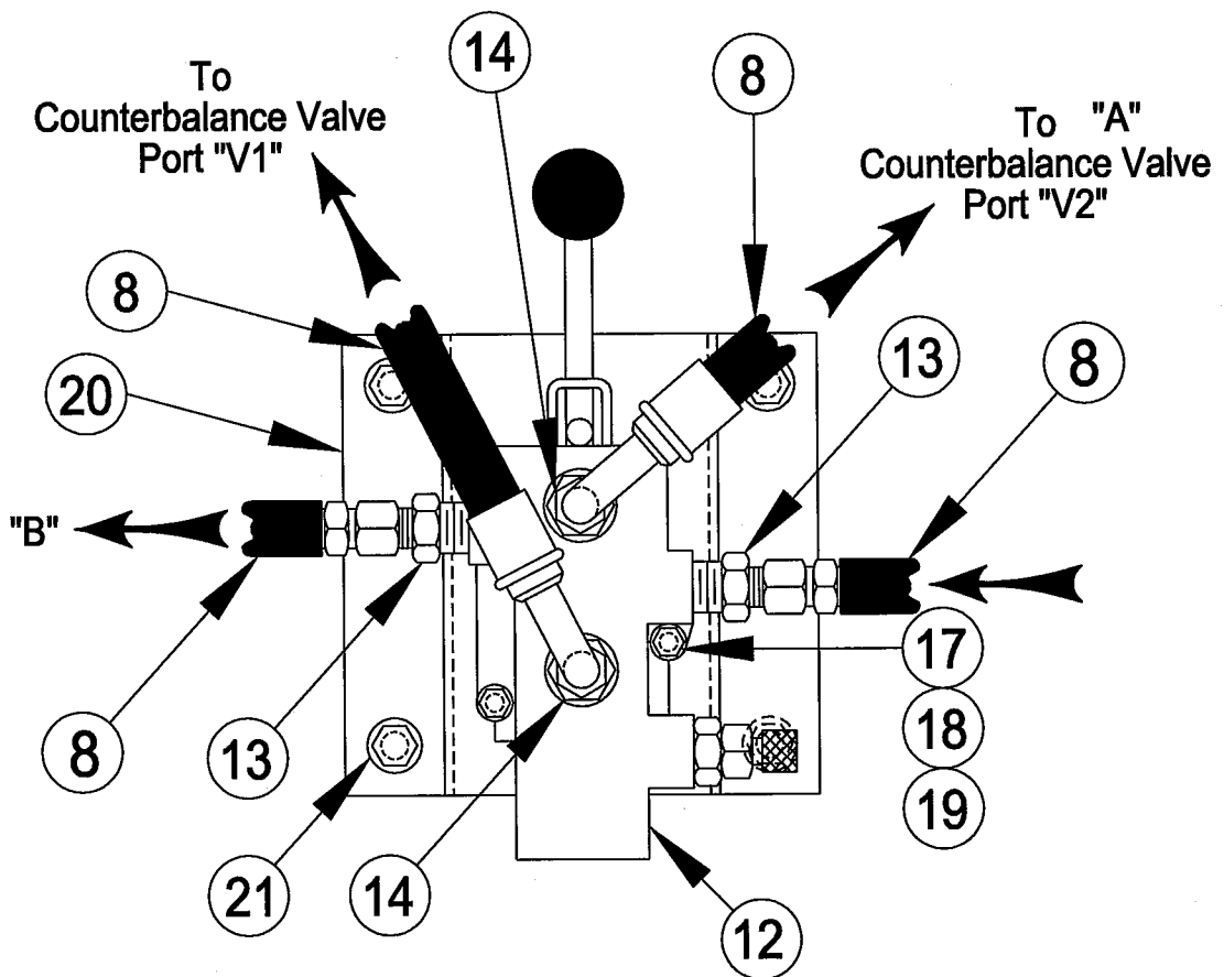
Hand Valve Assembly (Front View)
