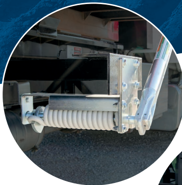
◀ 750 Fixed Undermount Spring
