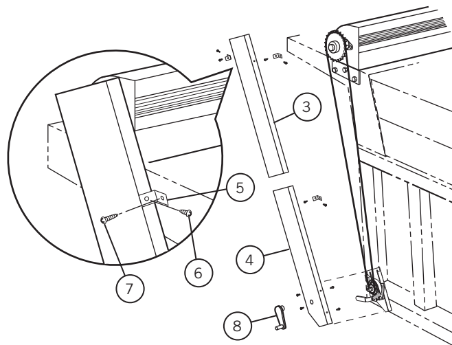
Aluminum Cover Figure 13-2
