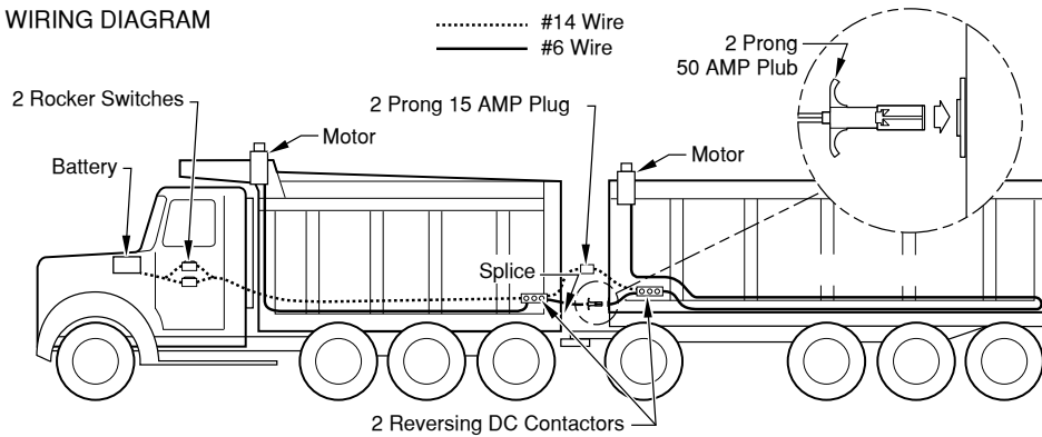
LEAD & PUP WIRING DIAGRAM
