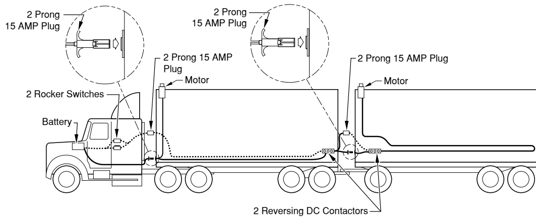
LEAD & PUP WIRING DIAGRAM
